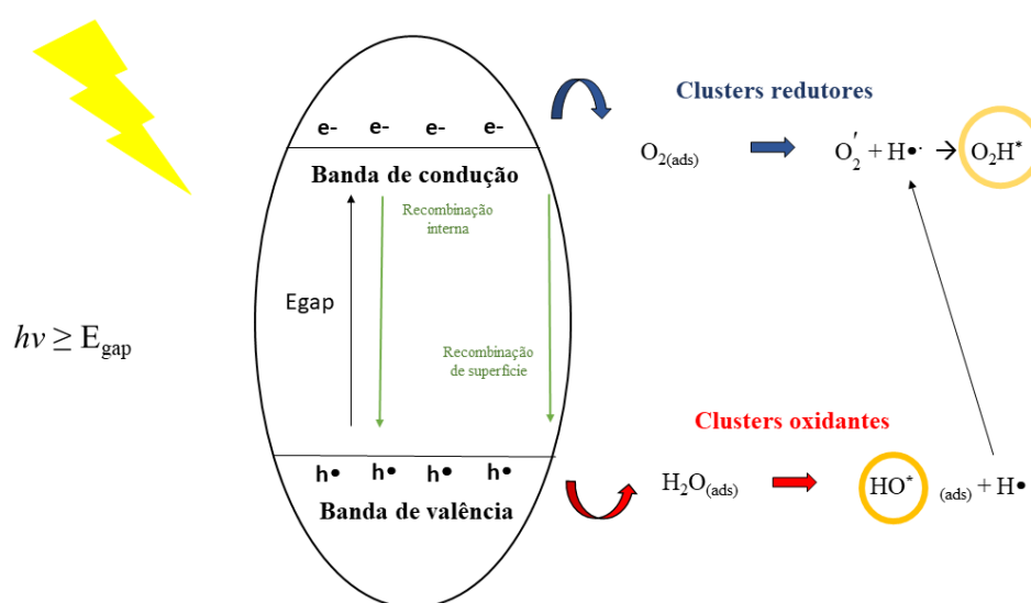
Figure 1 - Schematic representation of photocatalysis system.
