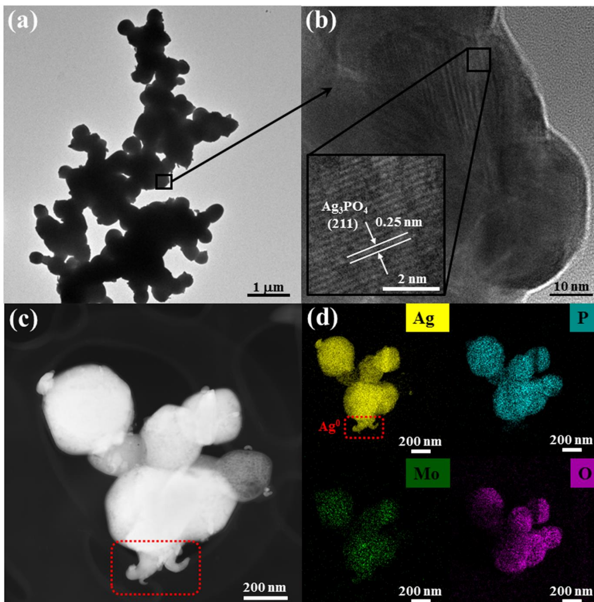
Figure 6 - TEM images of (a) \text{Ag}_3\text{PO}_4:\text{Mo} 2%, (b) characteristic interplanar distance of \text{Ag}_3\text{PO}_4 , (c) and (d) EDS maps of a group of particles in \text{Ag}_3\text{PO}_4:\text{Mo} 2%.
