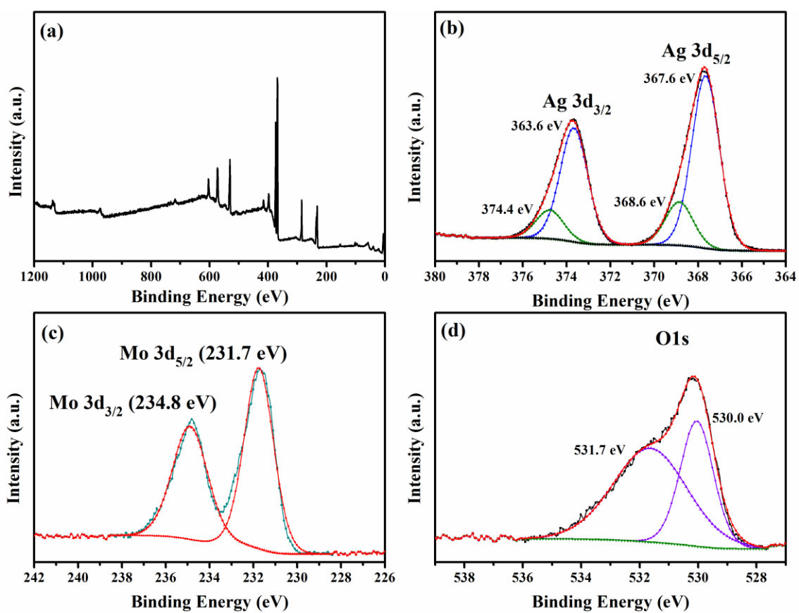
Figure SI-3. XPS spectra for pure \text{Ag}_2\text{MoO}_4 microcrystals. Survey spectra (a), Ag 3d (b), Mo 3d (c) and O 1s (d).
