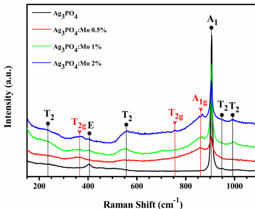
Figure 3 - Raman spectra of \text{Ag}_3\text{PO}_4 , \text{Ag}_3\text{PO}_4:\text{Mo} 0.5%, \text{Ag}_3\text{PO}_4:\text{Mo} 1%, and \text{Ag}_3\text{PO}_4:\text{Mo} 2%.
