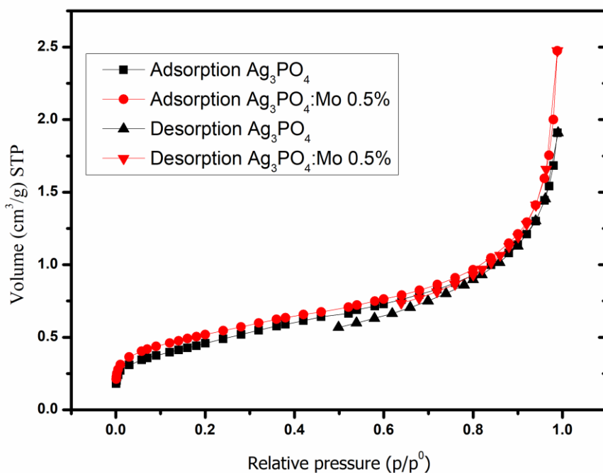
Figure SI-7. Adsorption-desorption isotherms of Size \text{Ag}_3\text{PO}_4 and \text{Ag}_3\text{PO}_4:\text{Mo} 0.5%.
