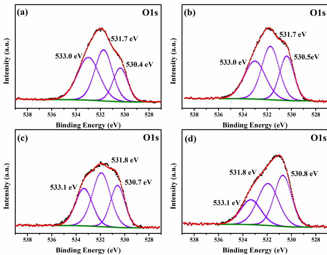
Figure SI-4. XPS spectrum of O 1s for pure \text{Ag}_3\text{PO}_4 (a), \text{Ag}_3\text{PO}_4 :Mo 0.5% (b), \text{Ag}_3\text{PO}_4 :Mo 1% (c) and \text{Ag}_3\text{PO}_4 :Mo 2% (d) samples.
