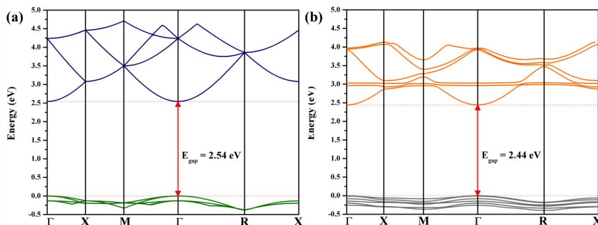
Figure 8 - The band structure of pure \text{Ag}_3\text{PO}_4 and \text{Ag}_3\text{PO}_4:\text{Mo} supercells.
