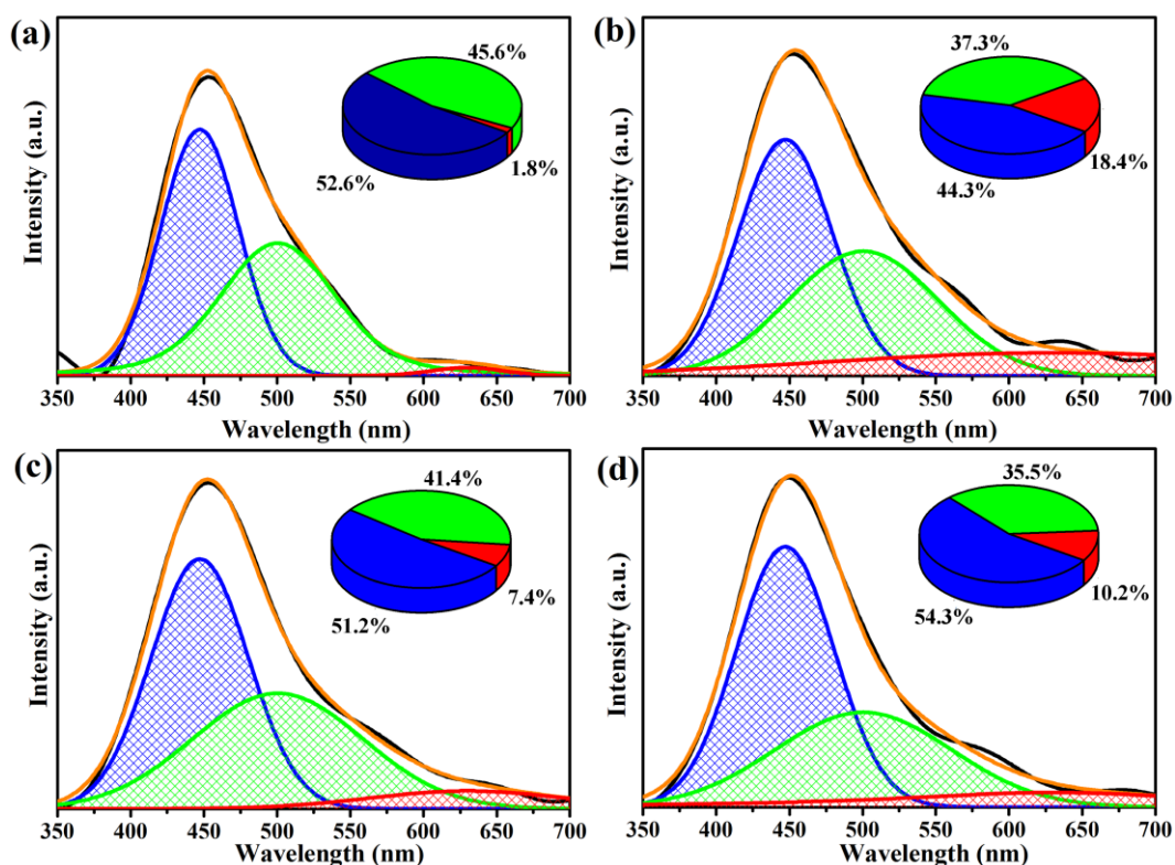
Figure 10 - Photoluminescence spectra (black line = experimental data) for (a) \text{Ag}_3\text{PO}_4 , (b) \text{Ag}_3\text{PO}_4:\text{Mo} 0.5%, (c) \text{Ag}_3\text{PO}_4:\text{Mo} 1% and (d) \text{Ag}_3\text{PO}_4:\text{Mo} 2%. Their deconvolution gives three peaks (orange line = sum), the distribution of them is given in inset.
