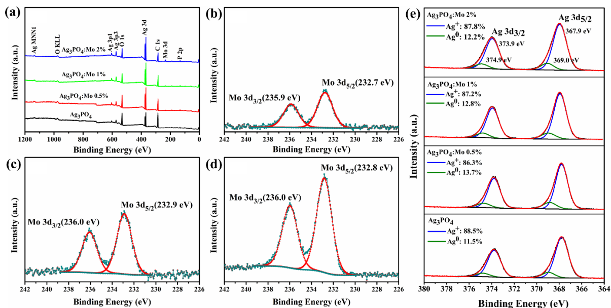
Figure 4 - XPS survey spectra of pure (black line) and \text{Mo}^{6+} doped (increasing amount from the bottom to top) \text{Ag}_3\text{PO}_4 microcrystals (a) and XPS spectrum of Mo 3d for \text{Ag}_3\text{PO}_4:\text{Mo} 0.5% (b), \text{Ag}_3\text{PO}_4:\text{Mo} 1% (c), \text{Ag}_3\text{PO}_4:\text{Mo} 2% (d) samples and (e) XPS spectra of Ag 3d for \text{Ag}_3\text{PO}_4 , \text{Ag}_3\text{PO}_4:\text{Mo} 0.5%, \text{Ag}_3\text{PO}_4:\text{Mo} 1% and \text{Ag}_3\text{PO}_4:\text{Mo} 2% samples.
