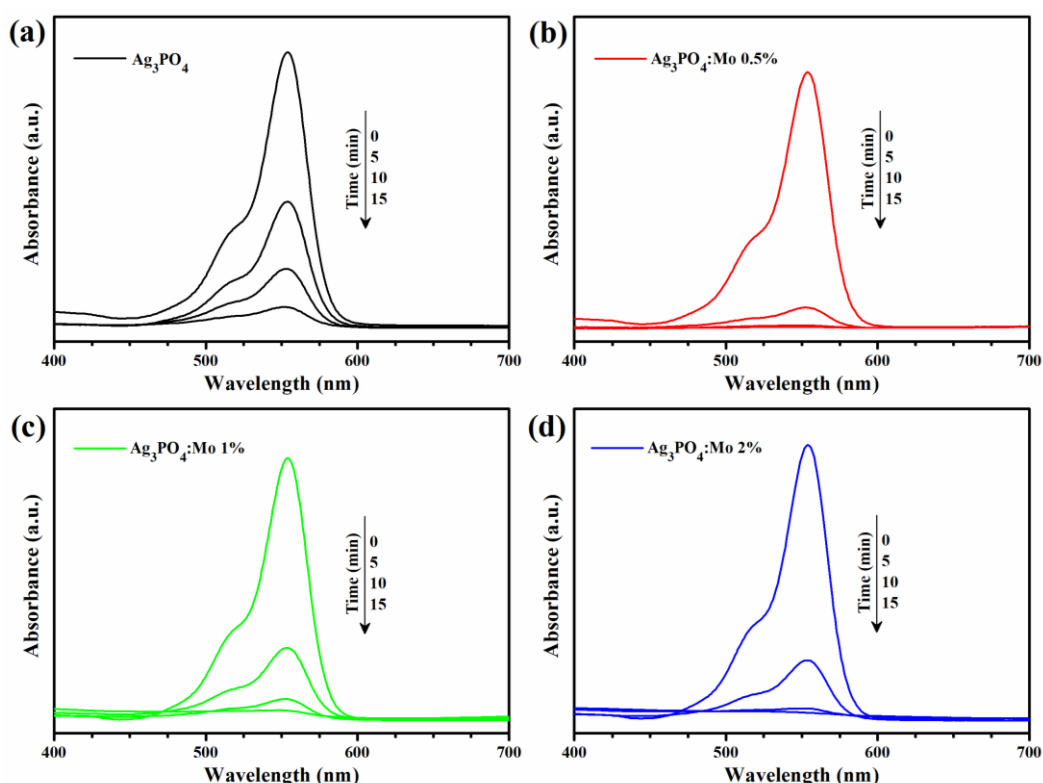
Figure 11 - UV-visible absorption spectra of RhB upon photodegradation in the presence of (a) \text{Ag}_3\text{PO}_4 , (b) \text{Ag}_3\text{PO}_4:\text{Mo} 0.5%, (c) \text{Ag}_3\text{PO}_4:\text{Mo} 1% and (d) \text{Ag}_3\text{PO}_4:\text{Mo} 2% catalysts.
