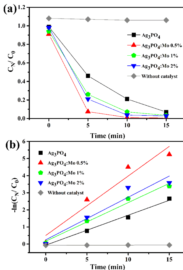
Figure 12 - Photocatalytic degradation of RhB ( 1.0 \times 10^{-5} mol L -1 ) in the absence and in the presence of Ag_3PO_4 and Ag_3PO_4 doped with different amounts of Mo in linear plot (a) and in log plot for the determination of the rate constant (b).
