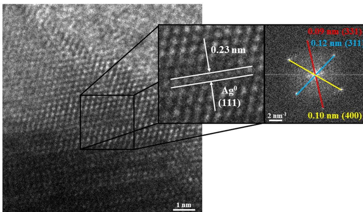
Figure 7 - HR-TEM images of the outgrowth visible on Figure 6 (c) and (d), showing a characteristic interplanar distance and the associated electron diffraction pattern.
