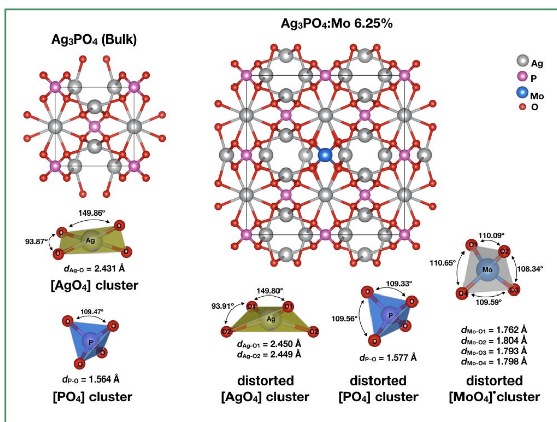
Figure 2 - Schematic representation of \text{Ag}_3\text{PO}_4 (bulk) and \text{Ag}_3\text{PO}_4:\text{Mo} supercell models.
