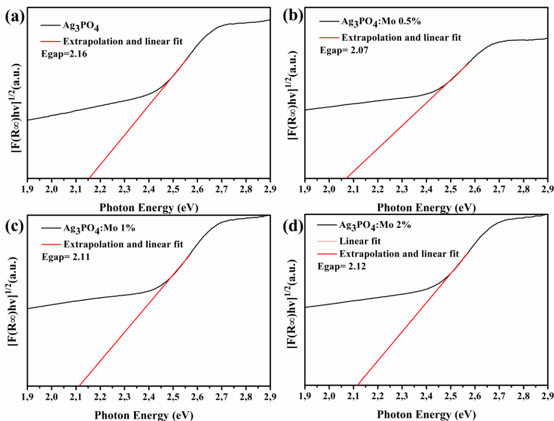
Figure SI-8. UV-visible absorption spectra and band gap energies for \text{Ag}_3\text{PO}_4 (a), \text{Ag}_3\text{PO}_4:\text{Mo} 0.5% (b), \text{Ag}_3\text{PO}_4:\text{Mo} 1% (c) and \text{Ag}_3\text{PO}_4:\text{Mo} 2% (d).
