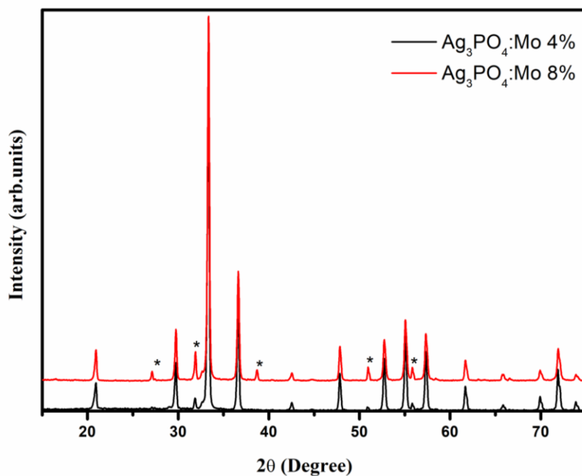
Figure SI-1. XRD patterns of overdoped samples \text{Ag}_3\text{PO}_4:\text{Mo} 4% and \text{Ag}_3\text{PO}_4:\text{Mo} 8%. Symbols * refer to \text{Ag}_2\text{MoO}_4 peaks.
