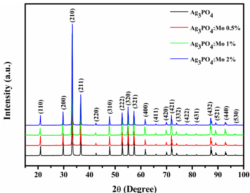
Figure 1 - XRD patterns of \text{Ag}_3\text{PO}_4 , \text{Ag}_3\text{PO}_4:\text{Mo} 0.5%, \text{Ag}_3\text{PO}_4:\text{Mo} 1%, and \text{Ag}_3\text{PO}_4:\text{Mo} 2%.
