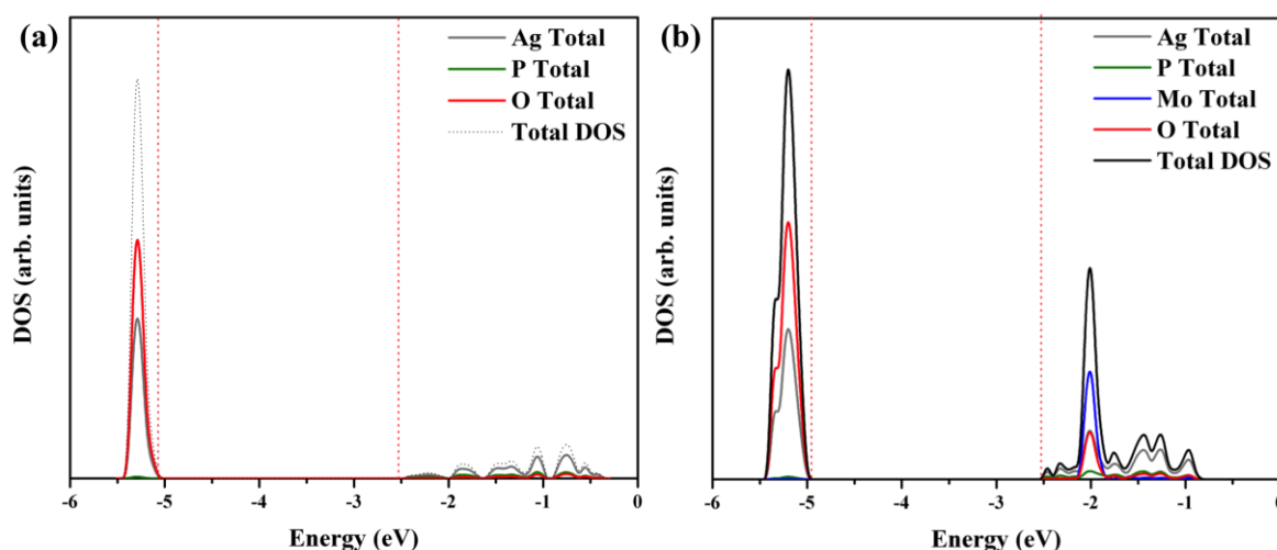
Figure 9 - The total DOS for the pure \text{Ag}_3\text{PO}_4 and \text{Ag}_3\text{PO}_4:\text{Mo} supercells.
